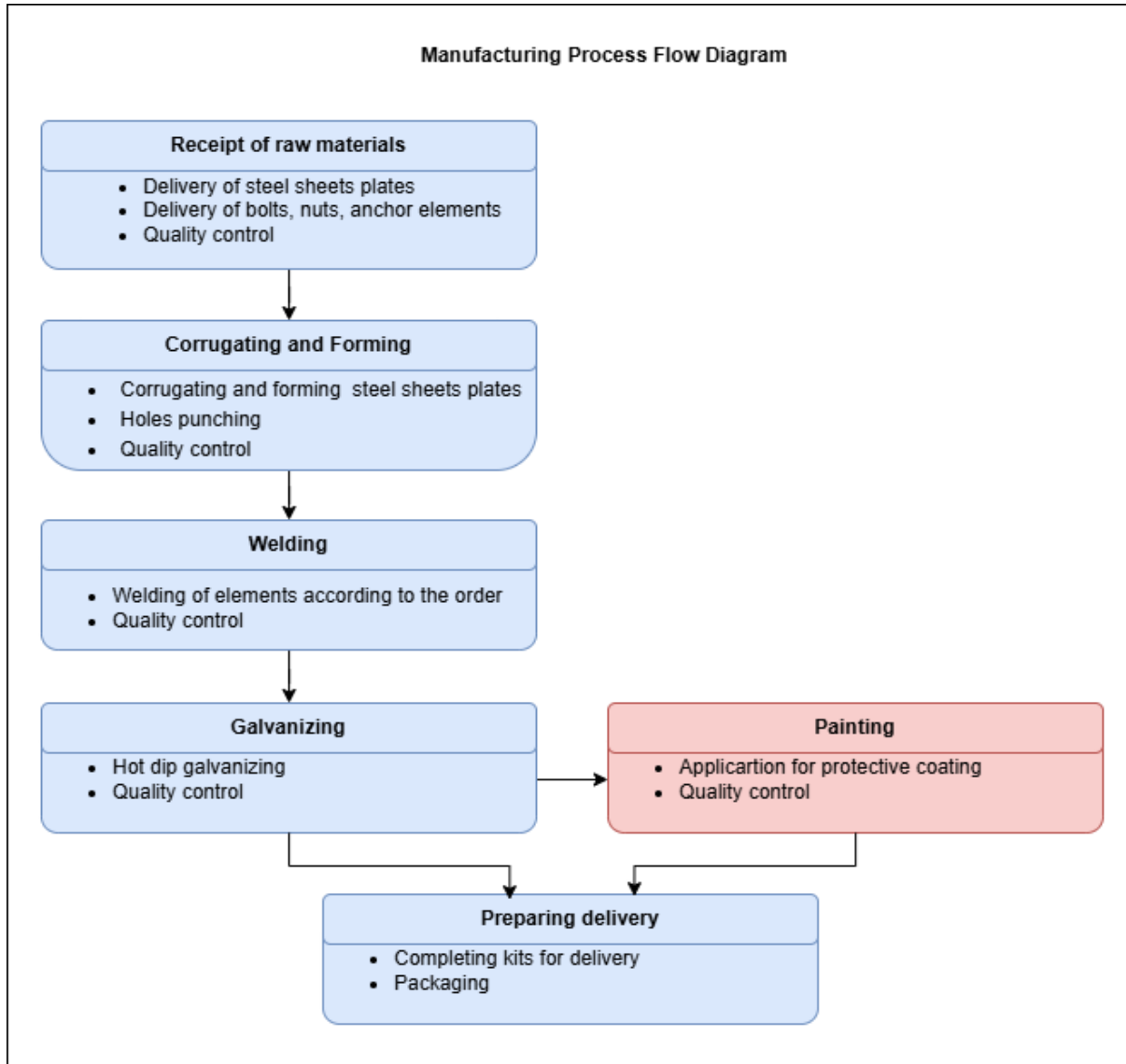
Figure 1 – Diagram of the manufacturing process
